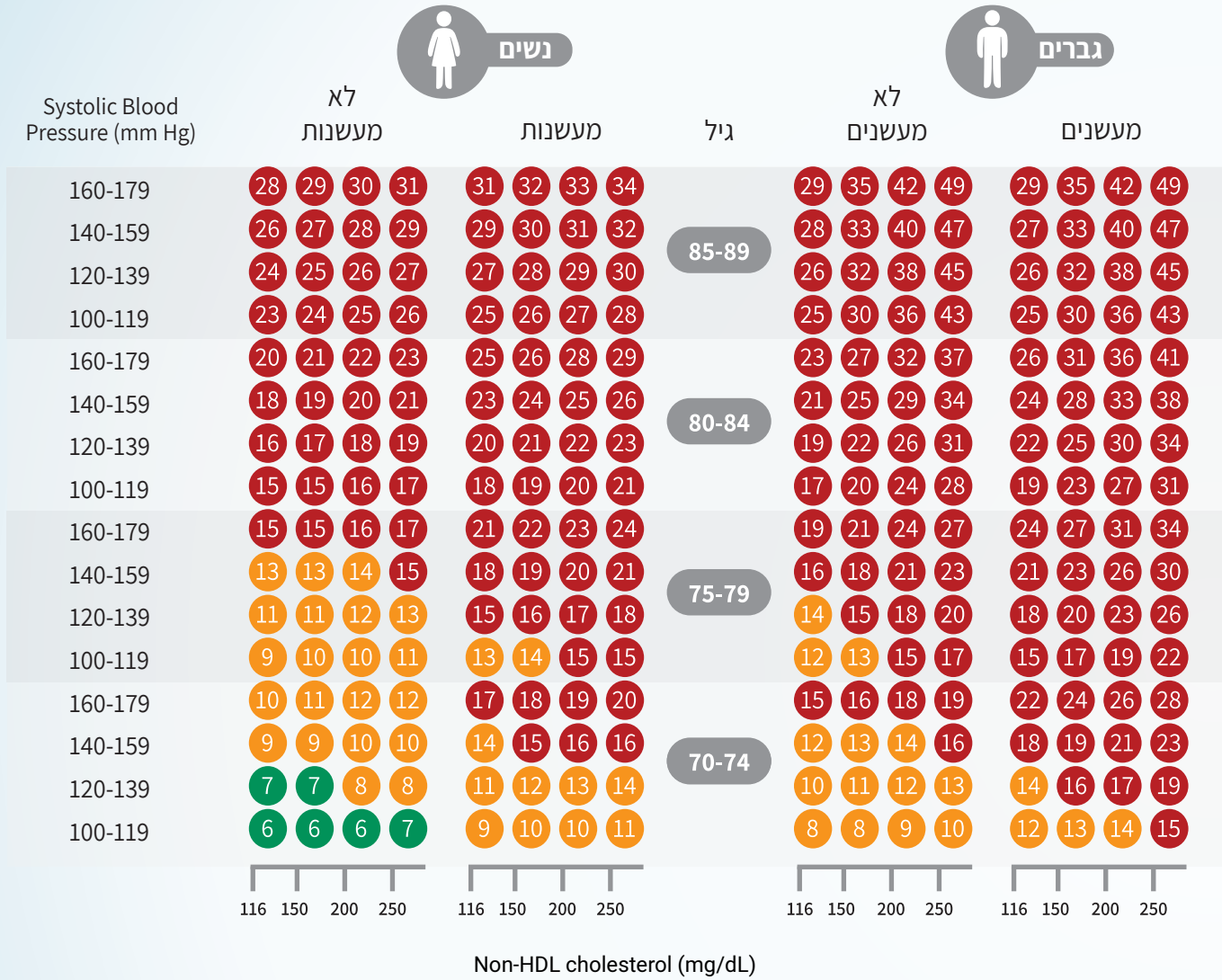
10 year risk of CV events in older persons in populations at low CVD risk
