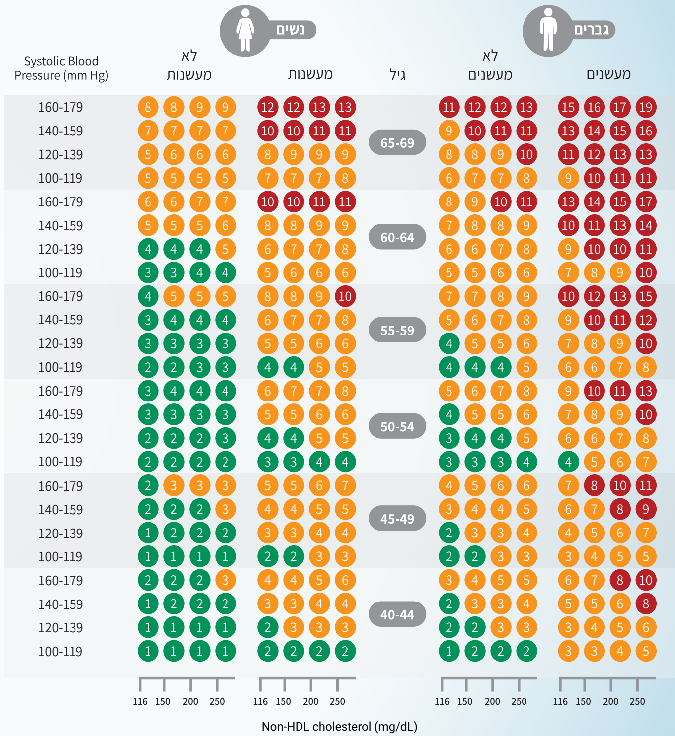
10 year risk of (fatal and non fatal) CV events in populations at low CVD risk
